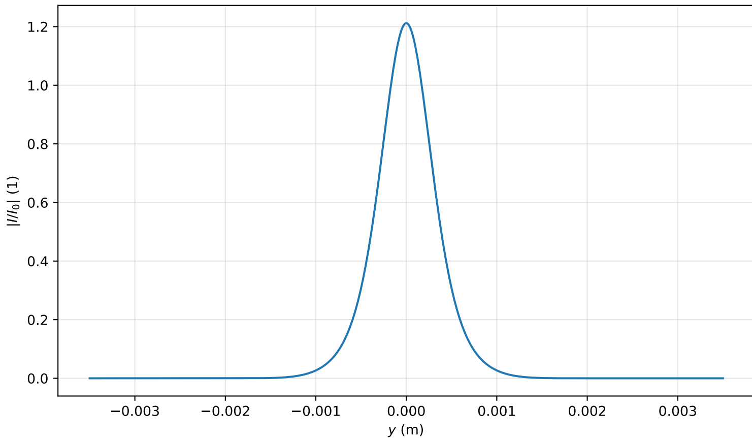
Intensity profile I(x=0, y, z=1.194)/I_0 , P_{in}=0.7P_{cr} , artificial time
